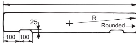
Wooden penboard
