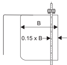
Rudder balance
