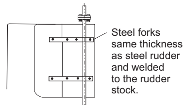
Wooden rudder
